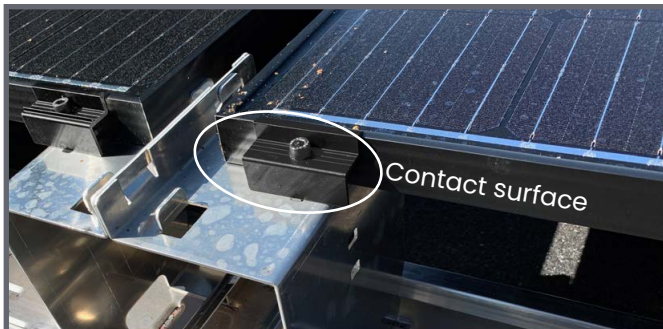
Distance 20 mm and contact surface
