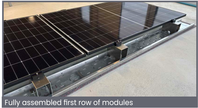
Fully assembled module supports for the first row of modules
