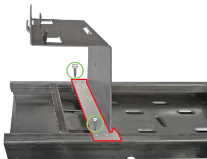
Duraklick mounting plate
